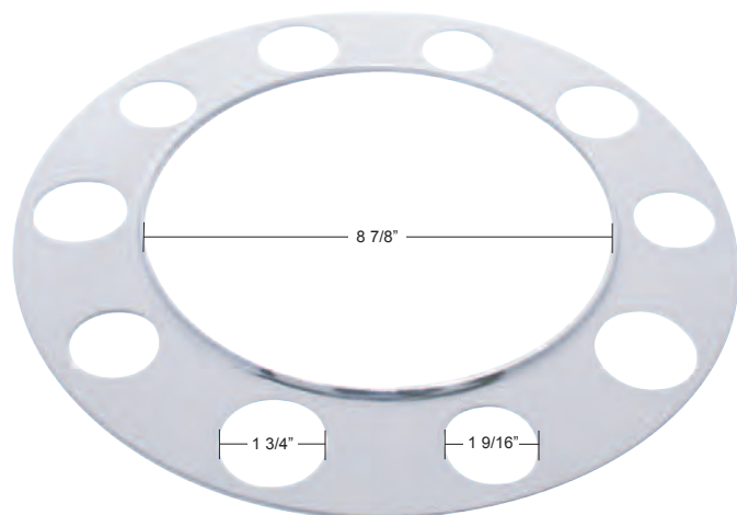
Stud Piloted / Steel Wheel
