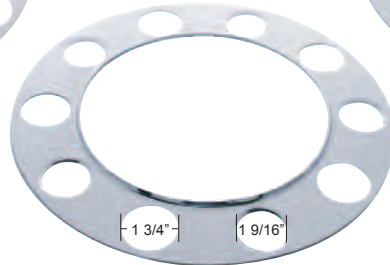
10215 Stud Piloted (Tapered) / Aluminum Wheel
